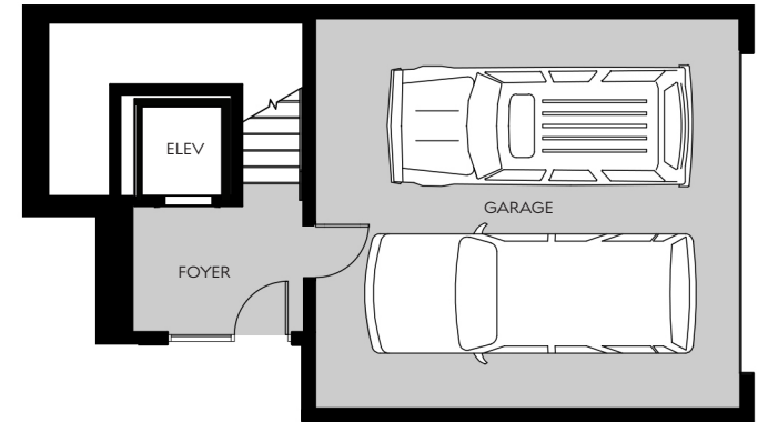
GROUND FLOOR - ENTRY
